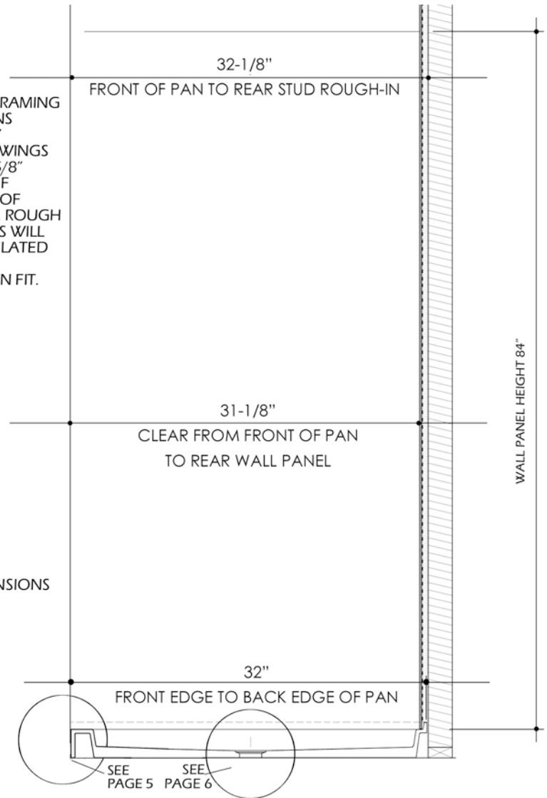
SIDE SECTION INSTALLATION
