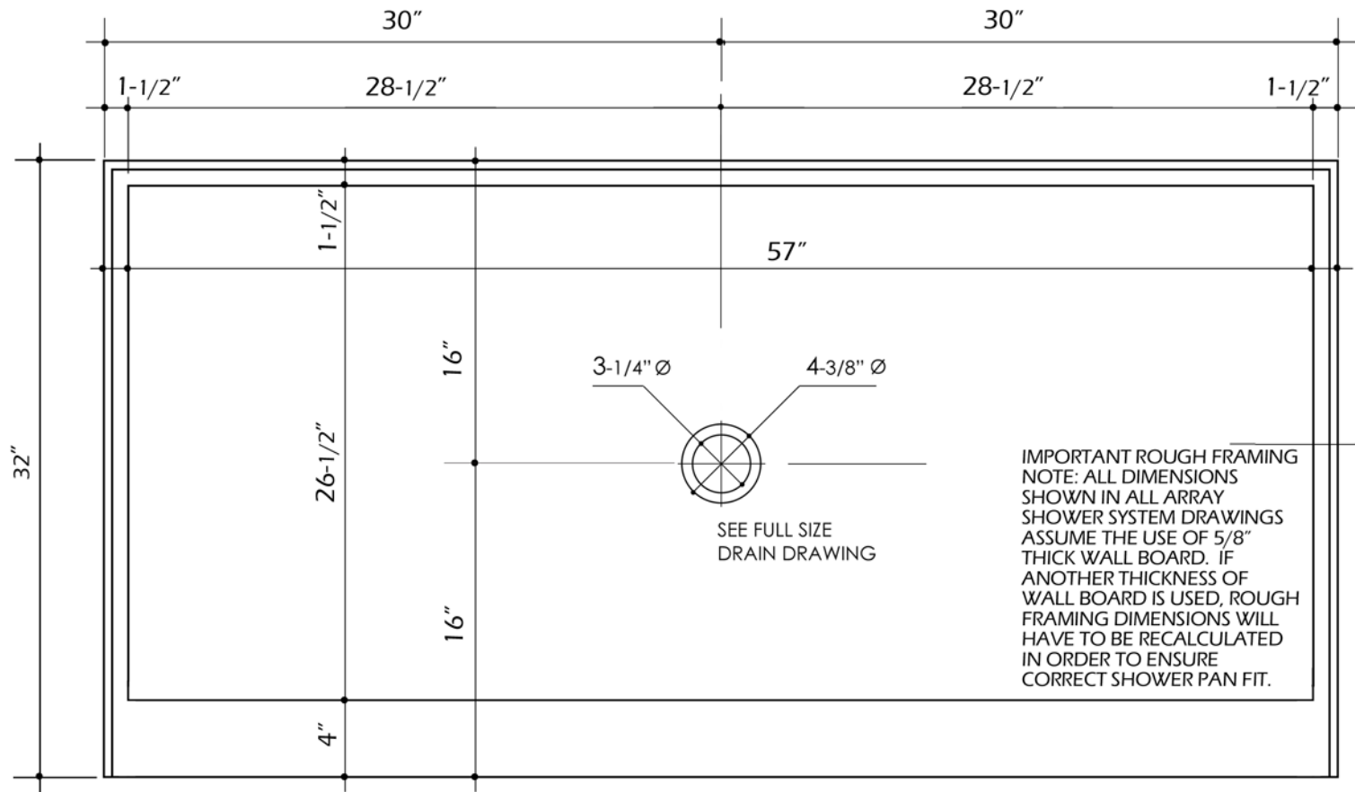
SP3260C SHOWER PAN DIMENSIONS 32"D X 60"W
