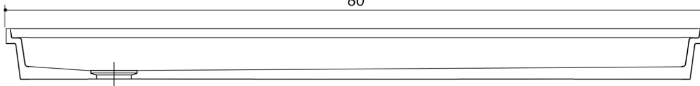
SP3260L SHOWER PAN DIMENSIONS 32"D X 60"W
