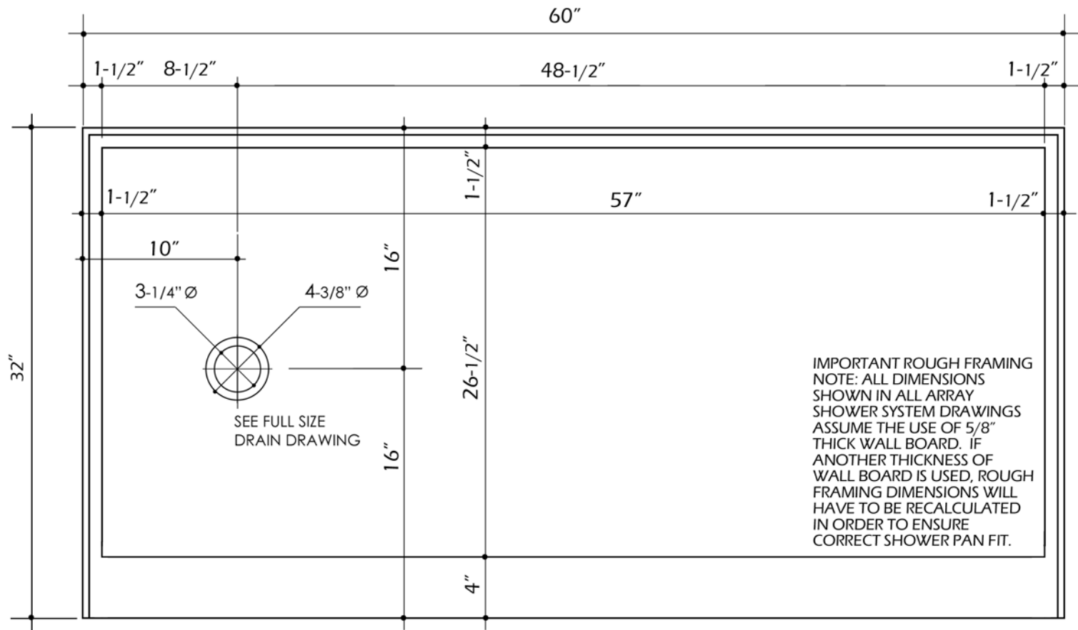
SP3260L SHOWER PAN DIMENSIONS 32"D X 60"W
