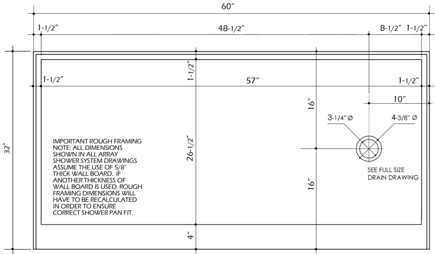
SP3260R SHOWER PAN DIMENSIONS 32"D X 60"W
