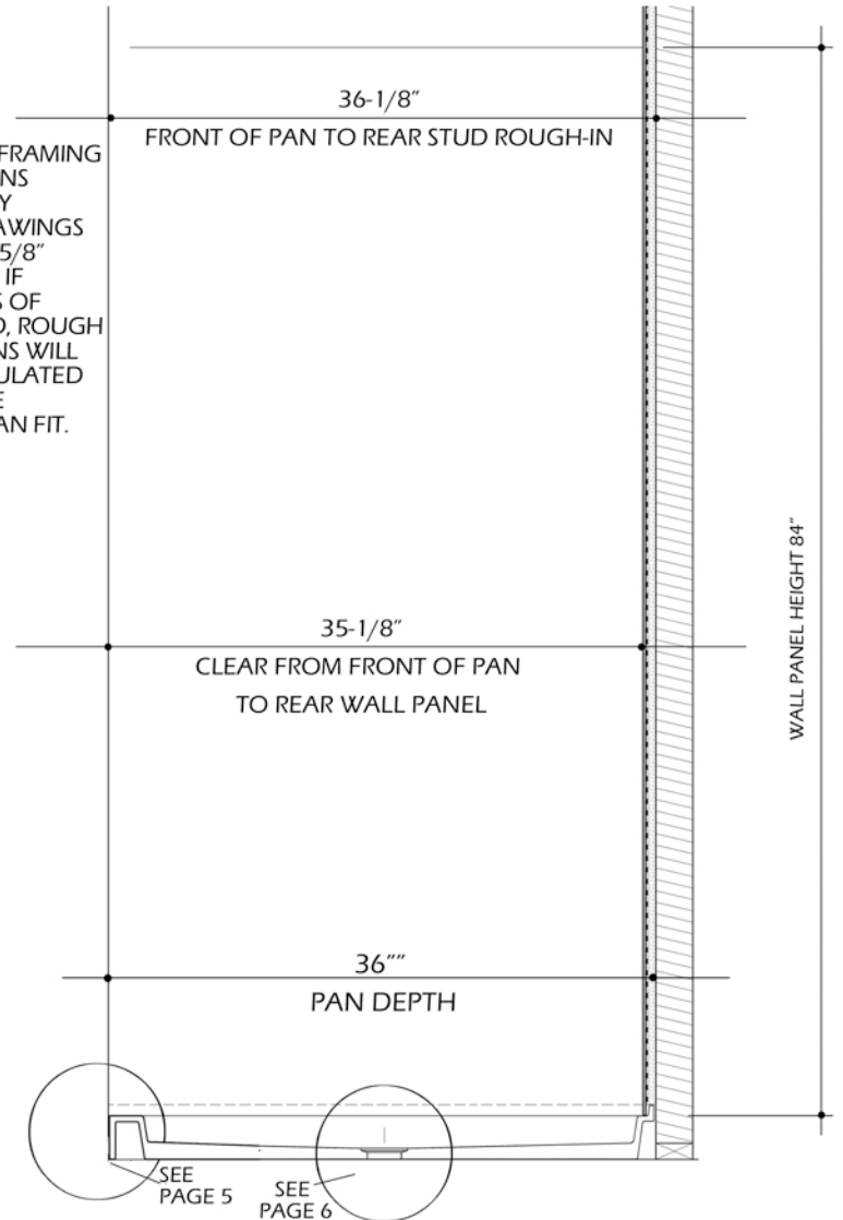
SECTION THROUGH SIDE OF SP3636 SHOWER PAN INSTALLATION
