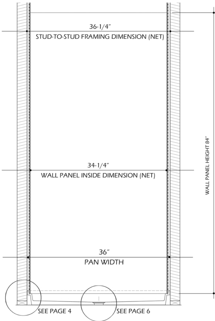
SECTION THROUGH FRONT OF SP3636 SHOWER PAN INSTALLATION
